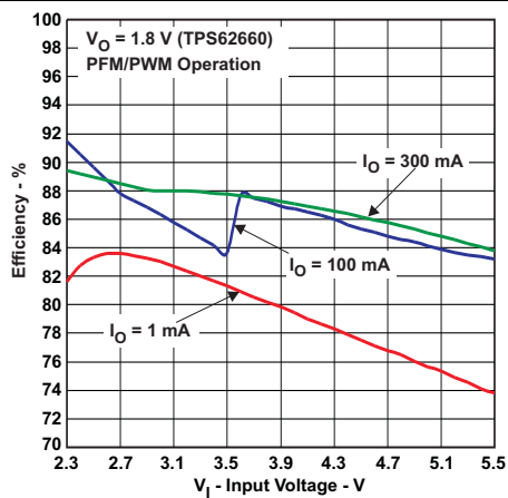
Figure 5. Efficiency vs Input Voltage
